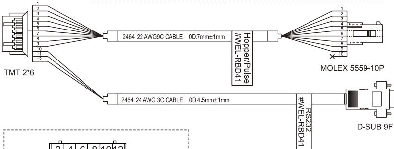
TMT 2*6 BACK VIEW
